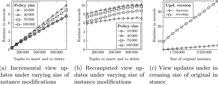
Fig. 5: Experimental runtime comparison of the incremental and the straightforward recomputation (of stage 2) version of the view update procedure
